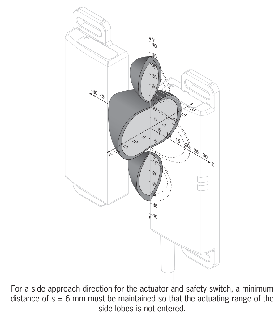
Fig. 4: Typical operating distance
