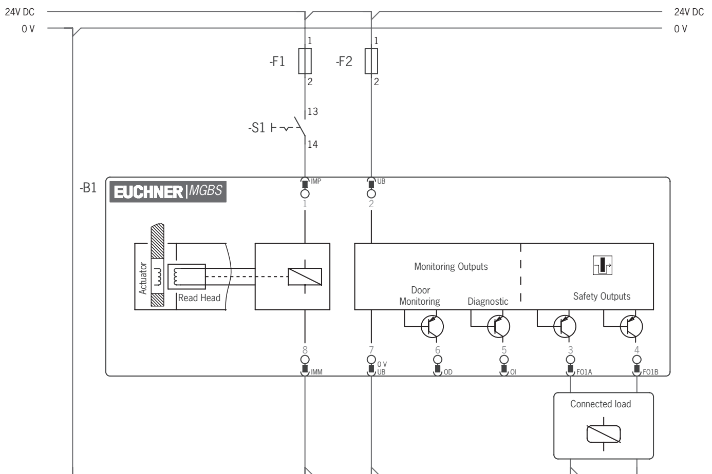
Fig. 4: Connection example, version with plug connector M12
