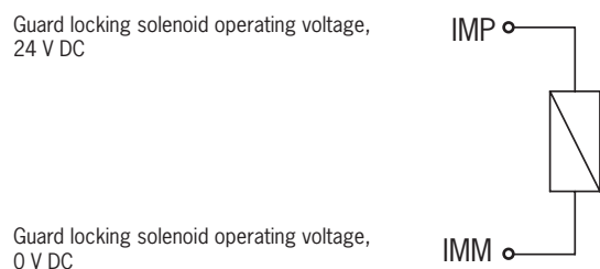
Fig. 6: Connection example with IMM connection
