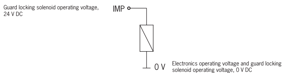
Fig. 7: Connection example without IMM connection
